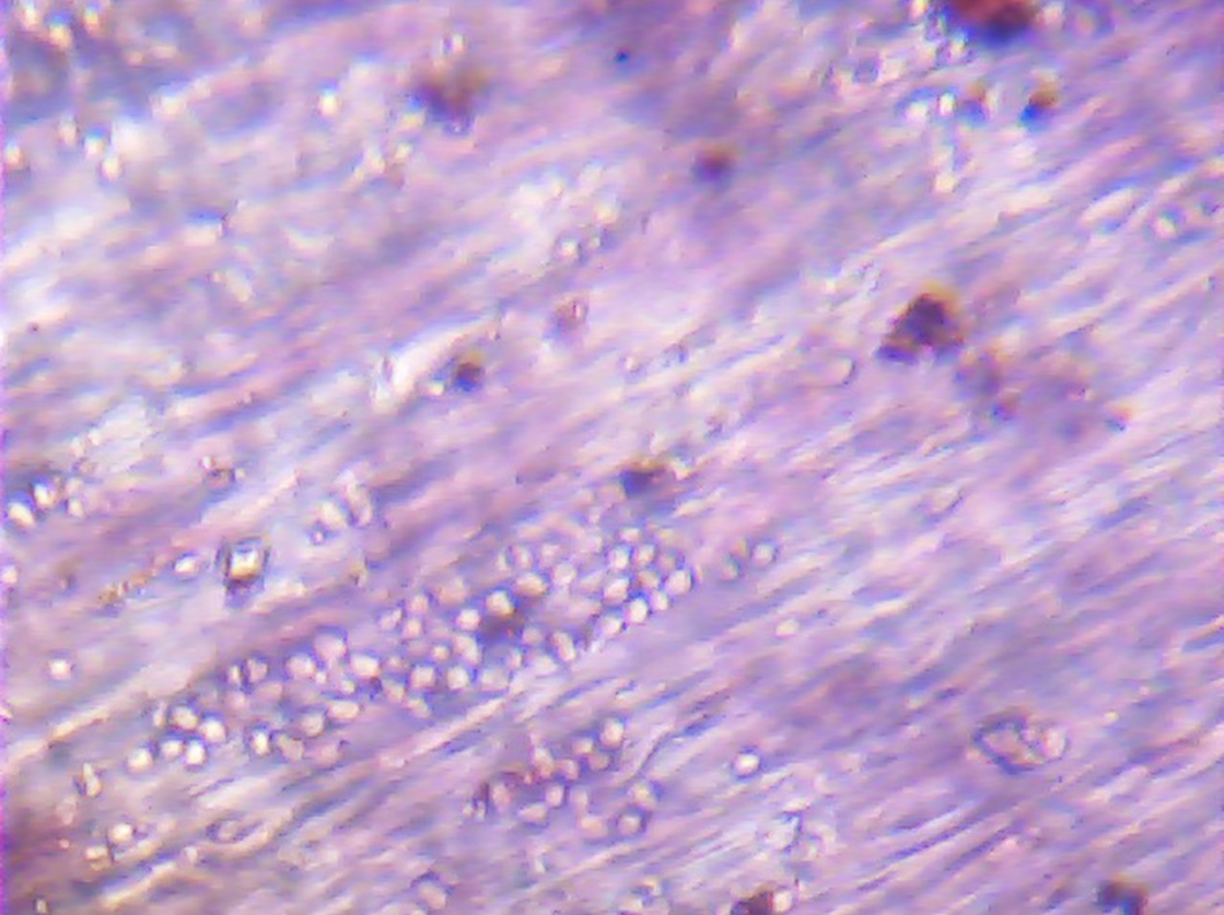
Statolithen
